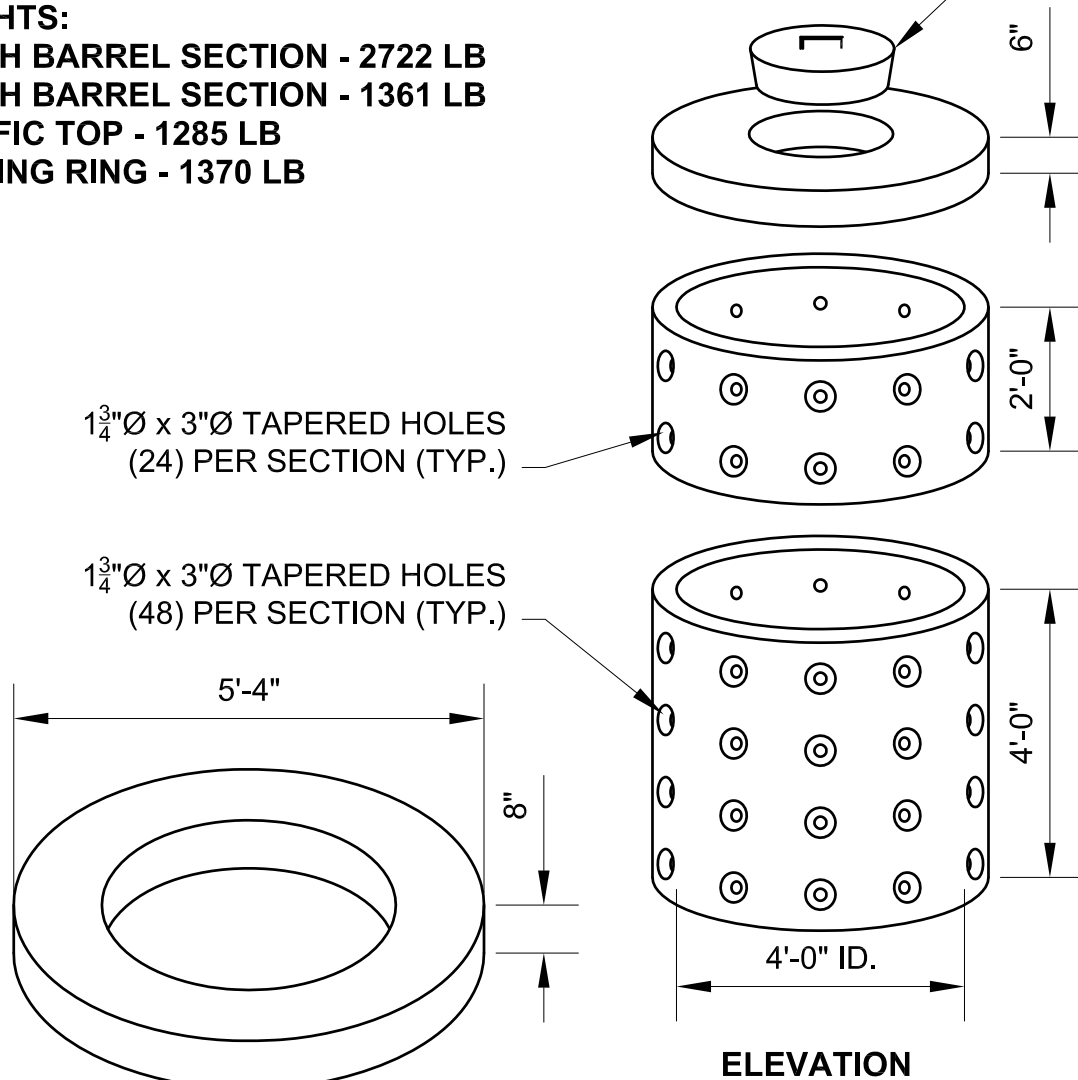
FOOTING RING
