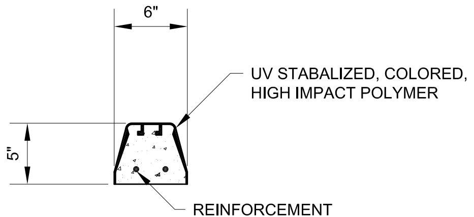
TYPICAL SECTION
