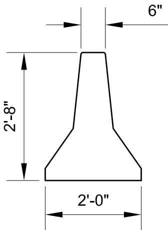
TYPICAL CROSS SECTION
