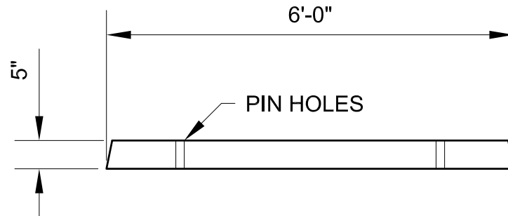
SIDE ELEVATION
